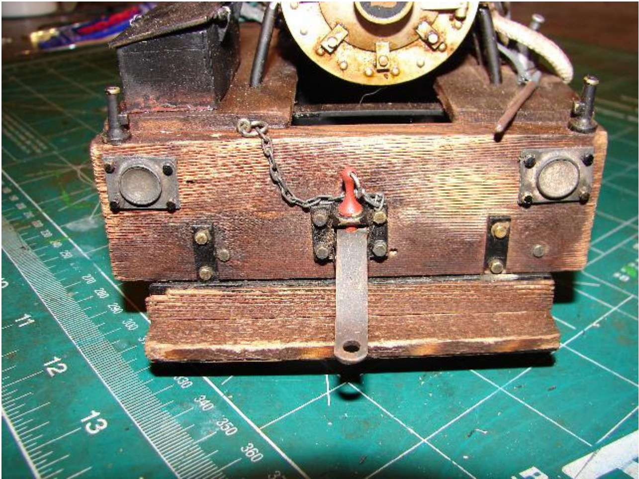
The other side has a steam driven punp for the siphon hose
